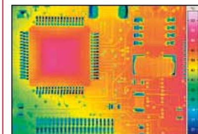
PCB, close-up image
